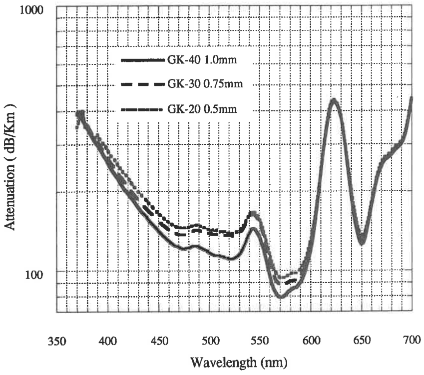
Figure 6.5 Effect of Fiber Diameter on Attenuation
