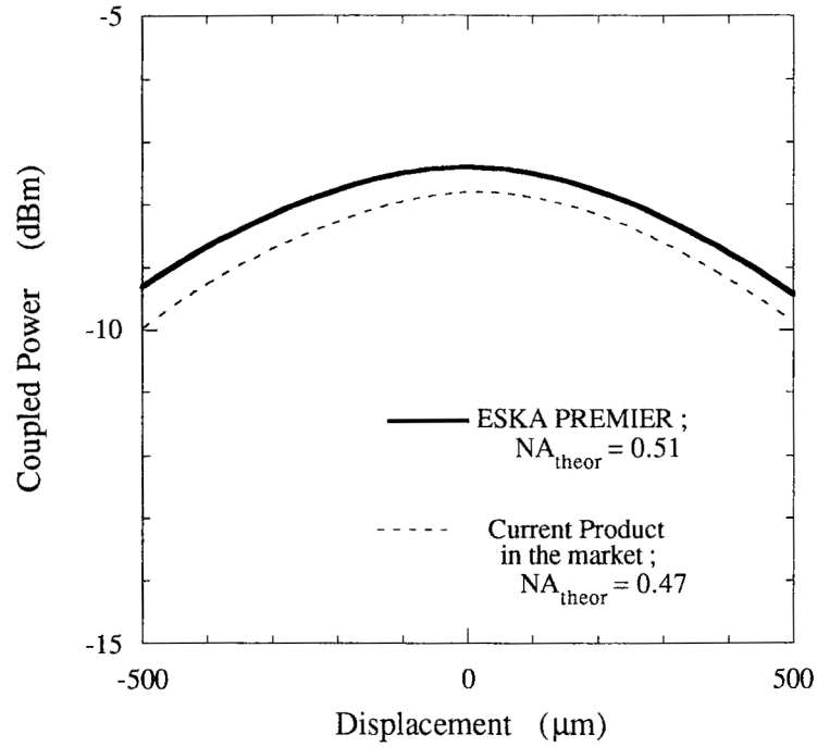
Figure 12.1 Axial Displacement
