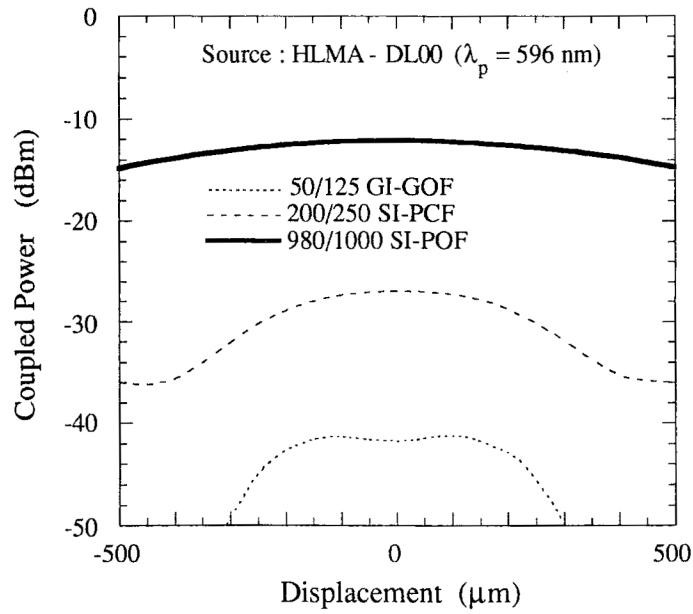
Figure 12.2 Comparison of Axial Displacement among Optical Fibers
