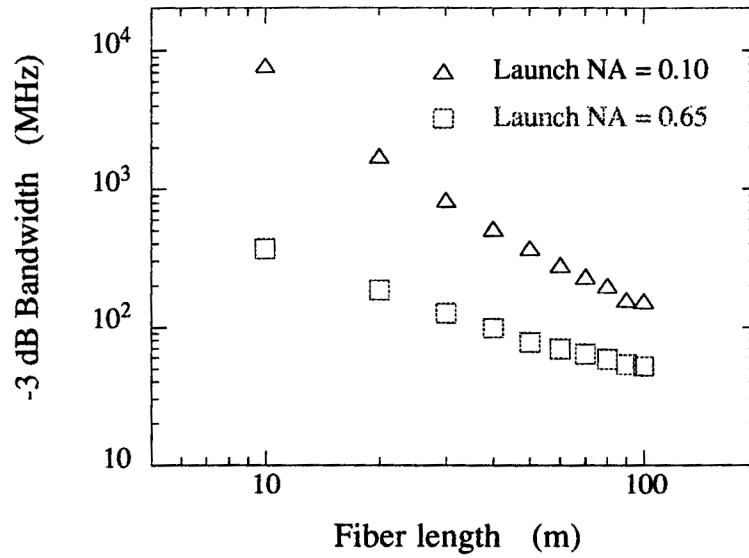
Figure 9.2 Measurements of Bandwidth
